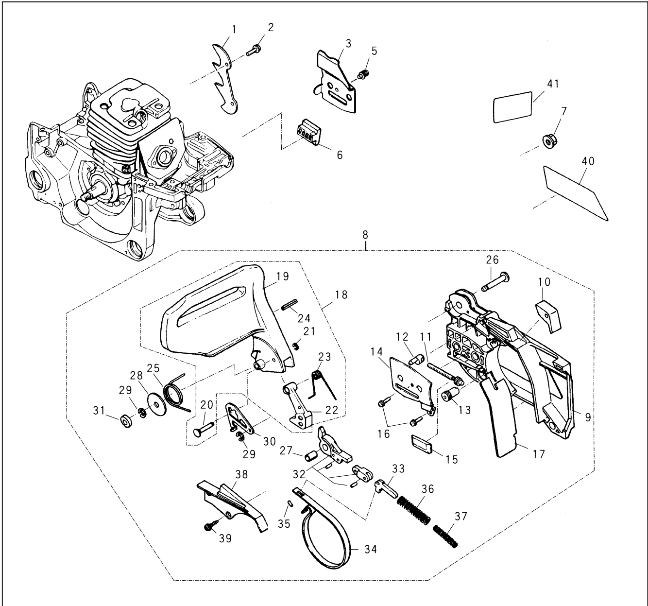
Fig.7 BAR MOUNT, CHAIN BRAKE
